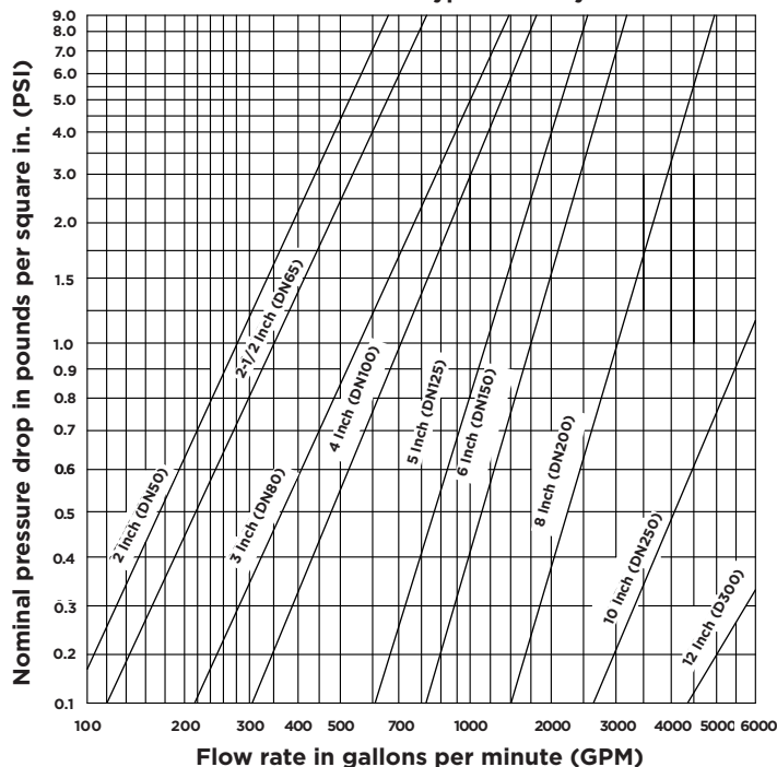
Friction Loss Wafer Type Butterfly Valve
