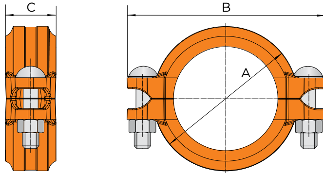
RIGID COUPLING STYLE 5
